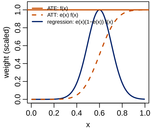
(c) weights by estimand
