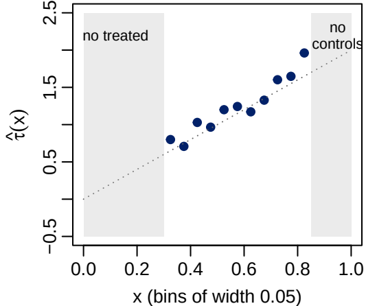
(b) bin-by-bin differences
