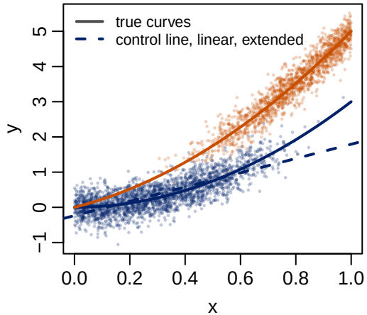
(a) data and a linear control fit
